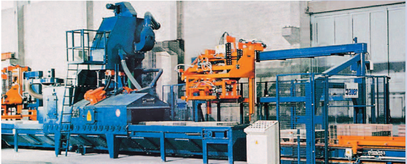
RST shot blasting line with automated handling and packaging
